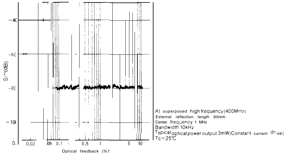
Fig. 78-1 S/N vs. Optical feedback
